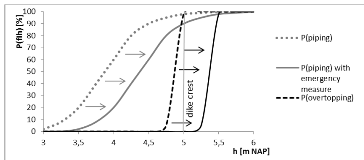
Figure 8: Potential effectiveness of overtopping (blue) and piping (green) measures
